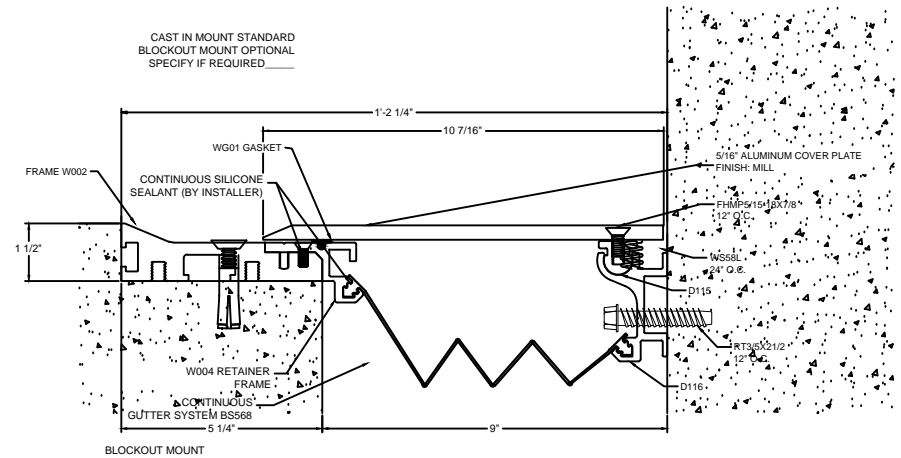
BLOCKOUT MOUNT
