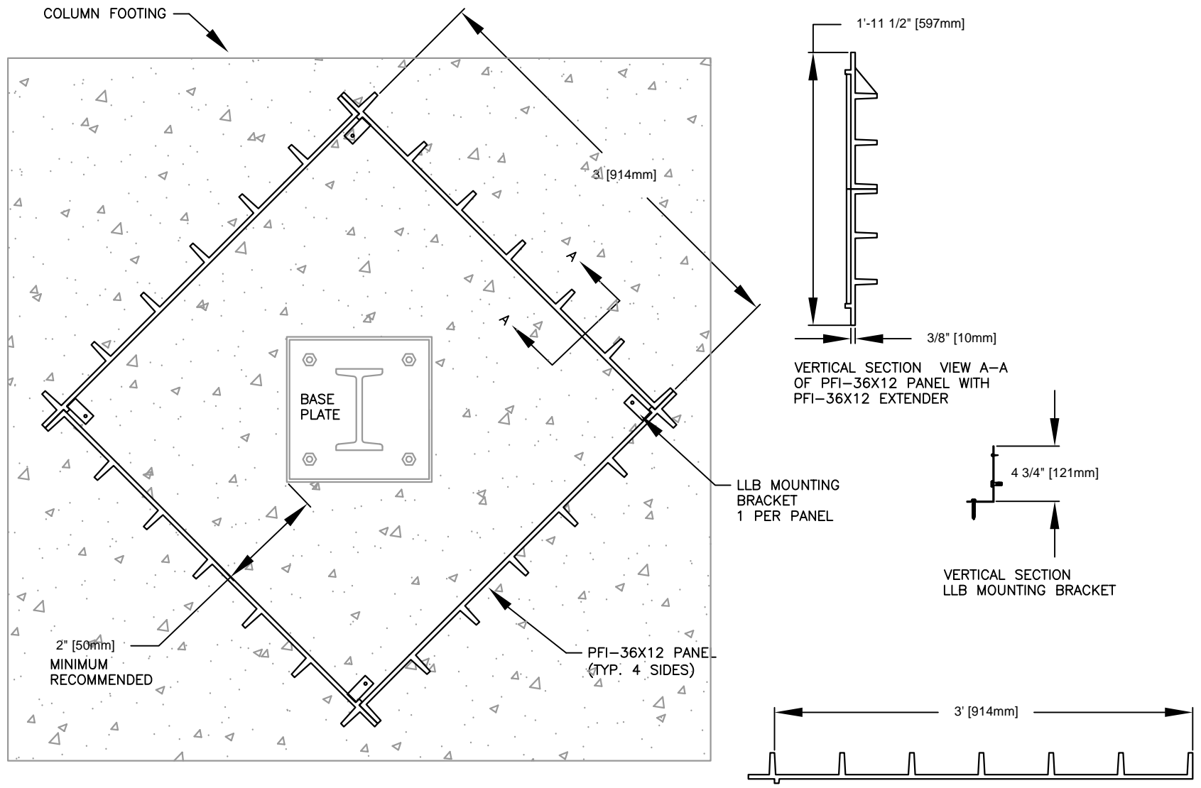
PLAN VIEW OF PFI-36X12 PANEL
