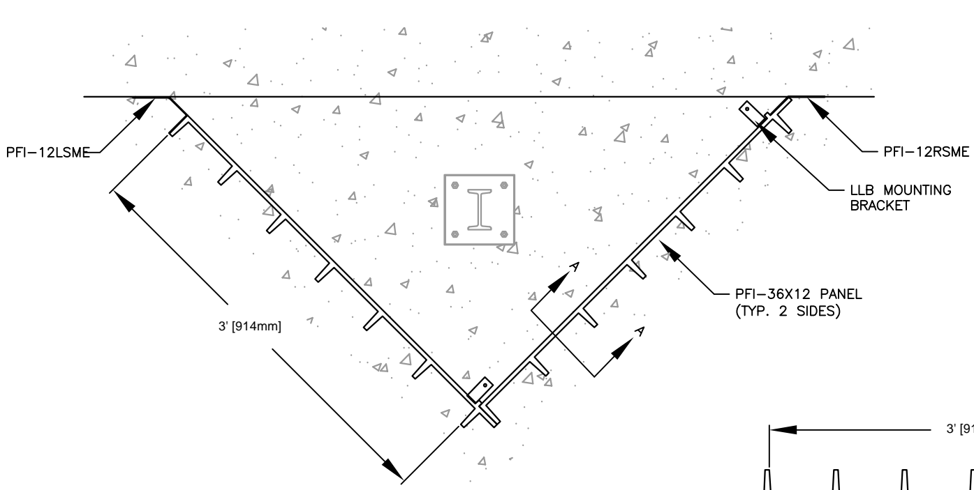
PLAN VIEW OF PFI-36X12 PANEL
