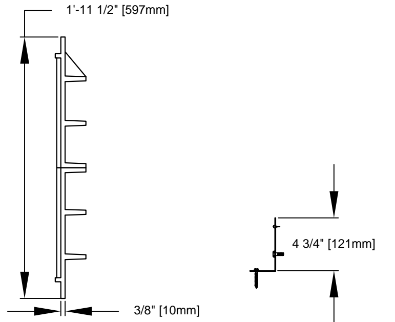
VERTICAL SECTION VIEW A-A OF PFI-36X12 PANEL WITH PFI-36X12 EXTENDER VERTICAL SECTION LLB MOUNTING BRACKET
