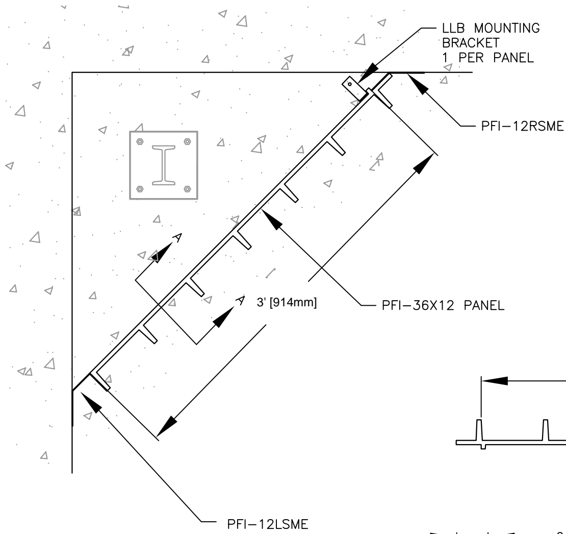
PLAN VIEW OF PFI-36X12 PANEL
