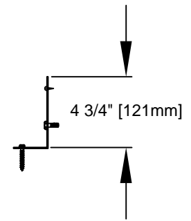
VERTICAL SECTION LLB MOUNTING BRACKET
