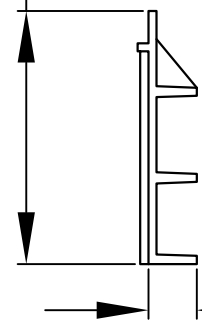
VERTICAL SECTION VIEW A-A OF PFI-36X12 PANEL
