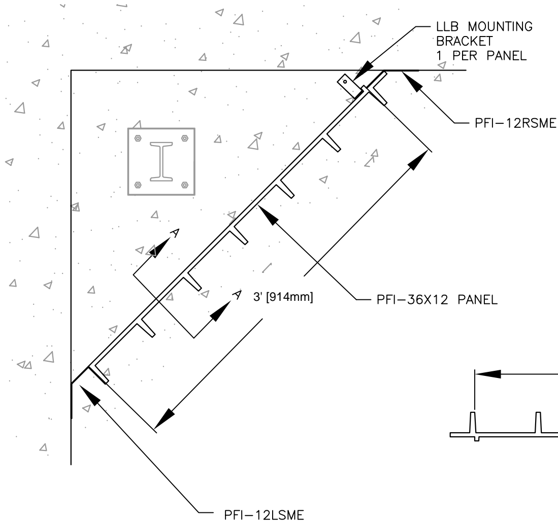
PLAN VIEW OF PFI-36X12 PANEL
