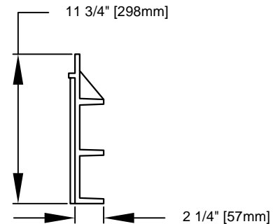
VERTICAL SECTION VIEW A-A OF PFI-28X12 PANEL
