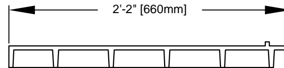
PLAN VIEW OF PFI-24X8 PANEL
