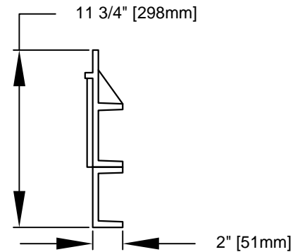
VERTICAL SECTION VIEW A-A OF PFI-24X8 PANEL WITH PFI-24X4 EXTENDER
