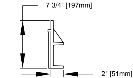
VERTICAL SECTION VIEW A-A OF PFI-24X8 PANEL
