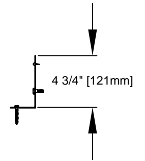
VERTICAL SECTION LLB MOUNTING BRACKET
